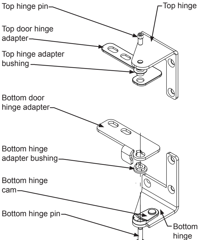
Figure 32 Right hand hinges shown
