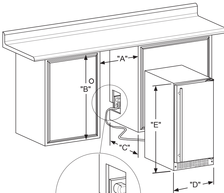
Figure 16 (S) Solid door shown
